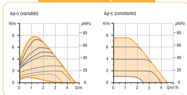
Circulator Halm modelo HEP Optimo Basic 25/8
