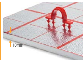
Grapa PS 10/16.
