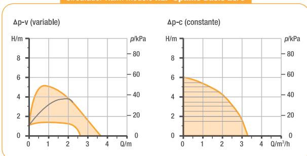
Circulator Halm modelo HEP Optimo Basic 25/6
